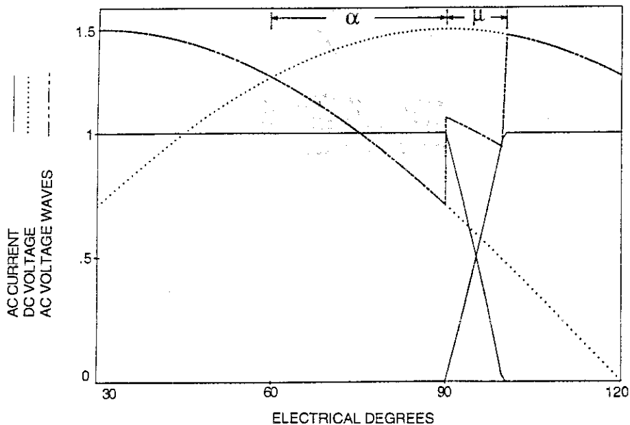
Fig 4.5 Commutation Overlap \alpha = 30^\circ , \mu = 12^\circ
