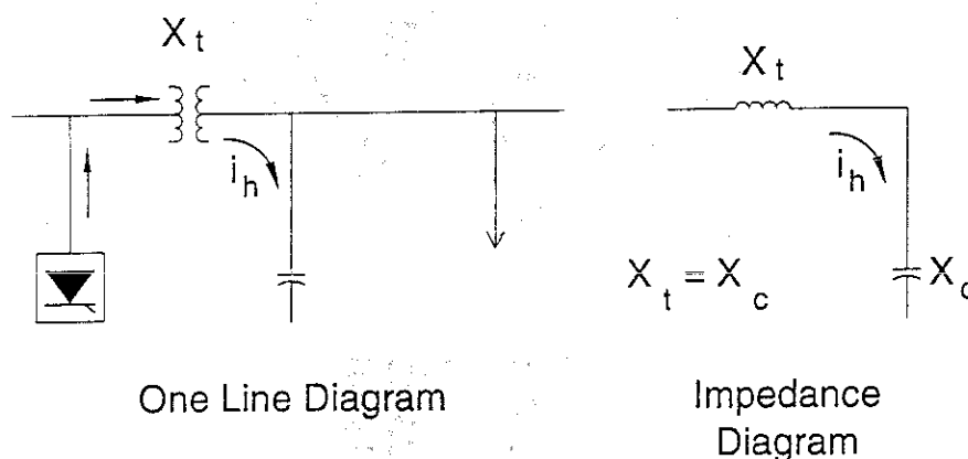
Fig 5.3 Capacitor Bank Resulting in Series Resonance
