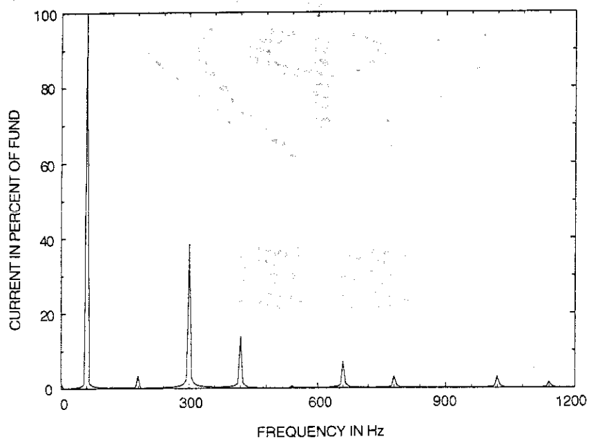
Fig 9.2 Spectrum Analyzer — Frequency Domain
