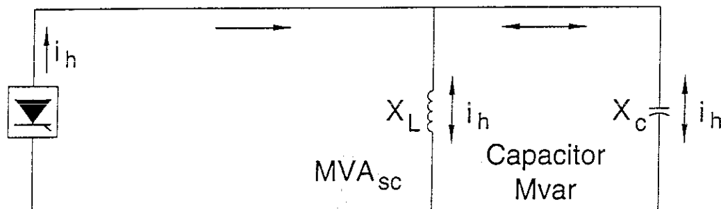
Fig 8.2 Simple Circuit for Hand Calculations
