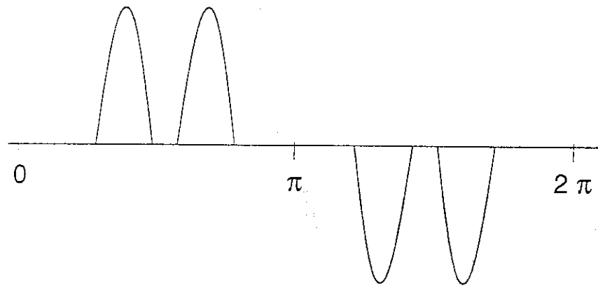
Fig 4.14 Current Wave of PWM Six-Pulse Power Supply Under Light Load (Discontinuous Current)
