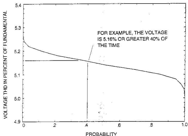
Fig 9.4 Harmonic Distribution Curve of Voltage THD
