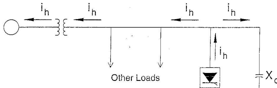
Fig 5.1 Normal Flow of Harmonic Currents
