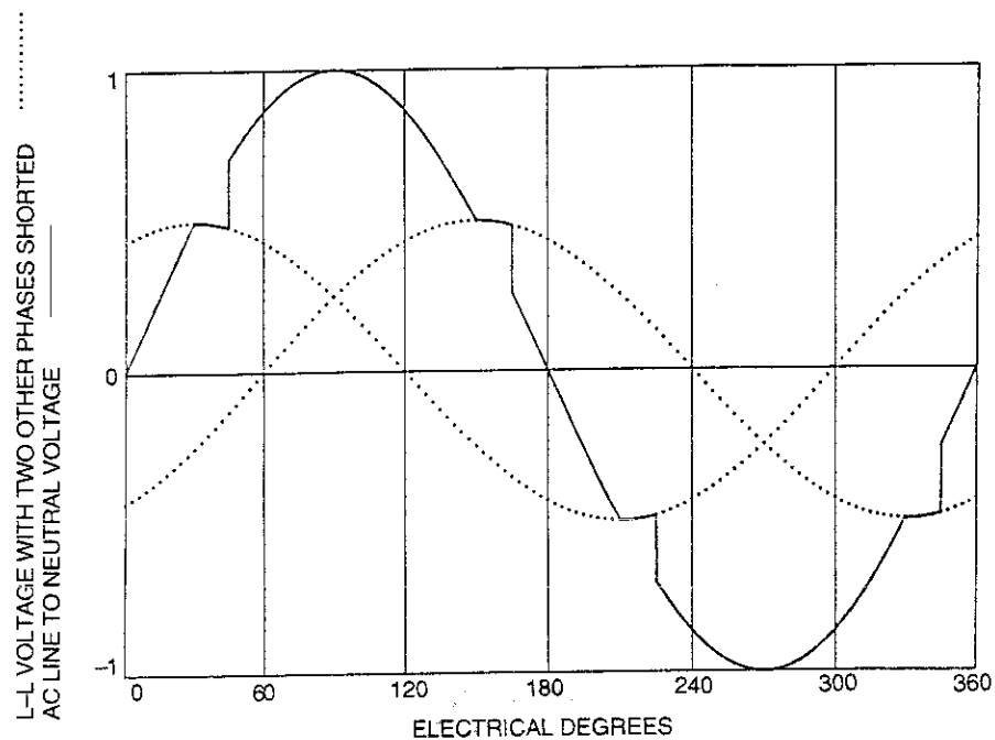
Fig 4.6 Rectifier Voltage Notching \alpha = 0^\circ
