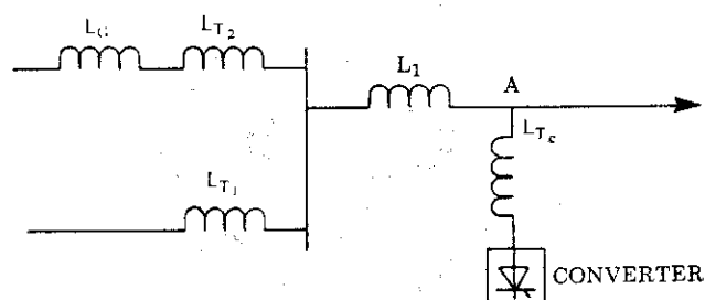
(b) Impedance Diagram
