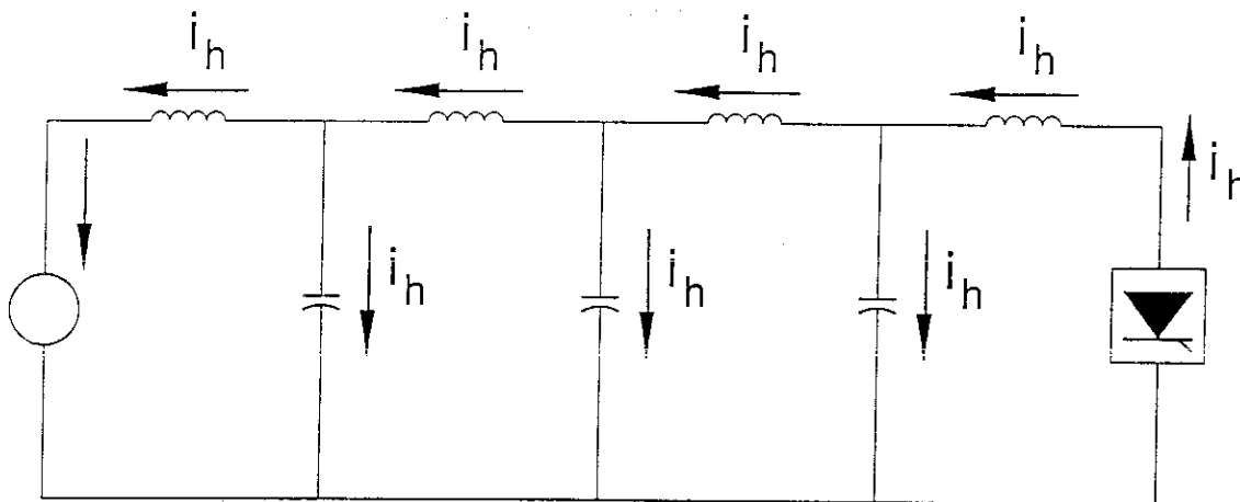
Fig 8.3 Long Line Equivalent Circuit
