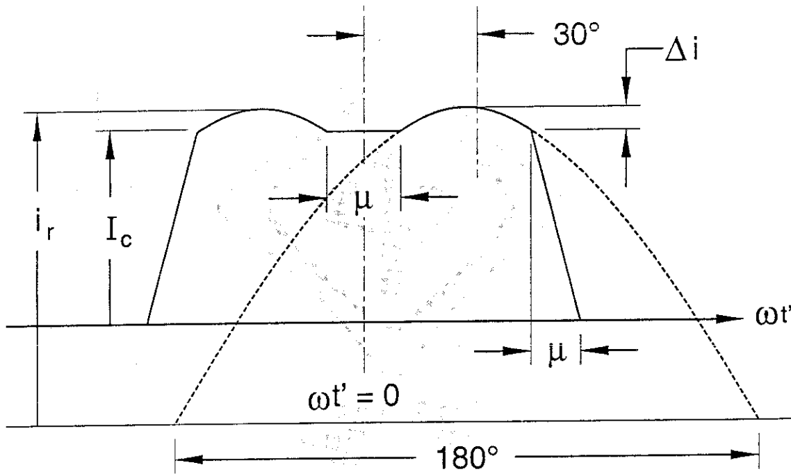
Fig 4.12 Definition of Values in Eq 4.9
