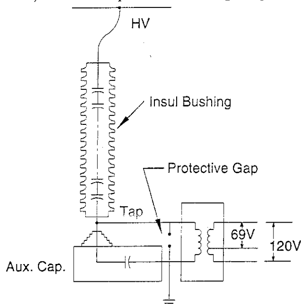
Fig 9.7 Capacitive Voltage Divider
