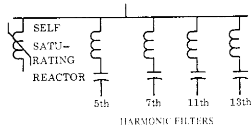
Fig 7.9 Reactive Power Compensation Using Saturable Reactor
