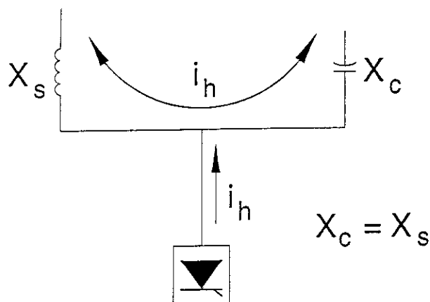
Fig 5.2 Parallel Resonance Condition
