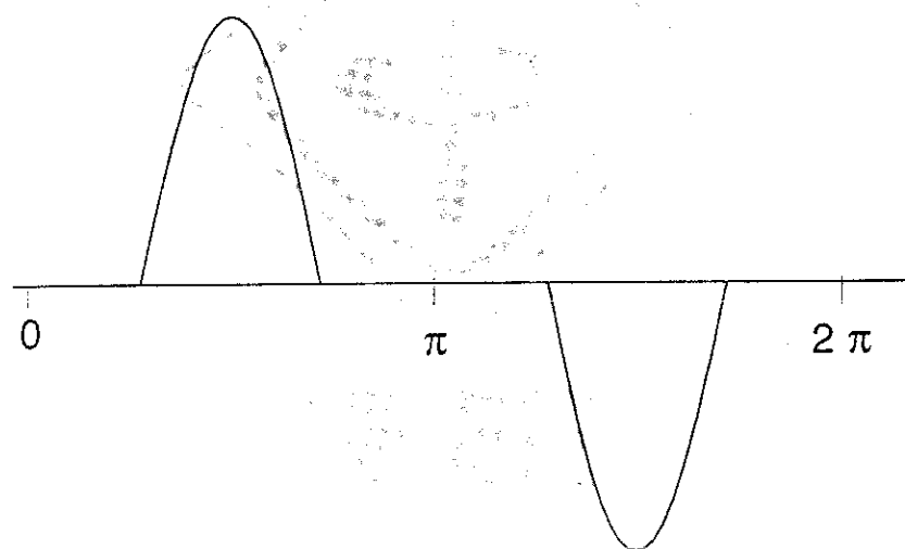
Fig 4.13 Current Wave of Switch Mode Power Supply
