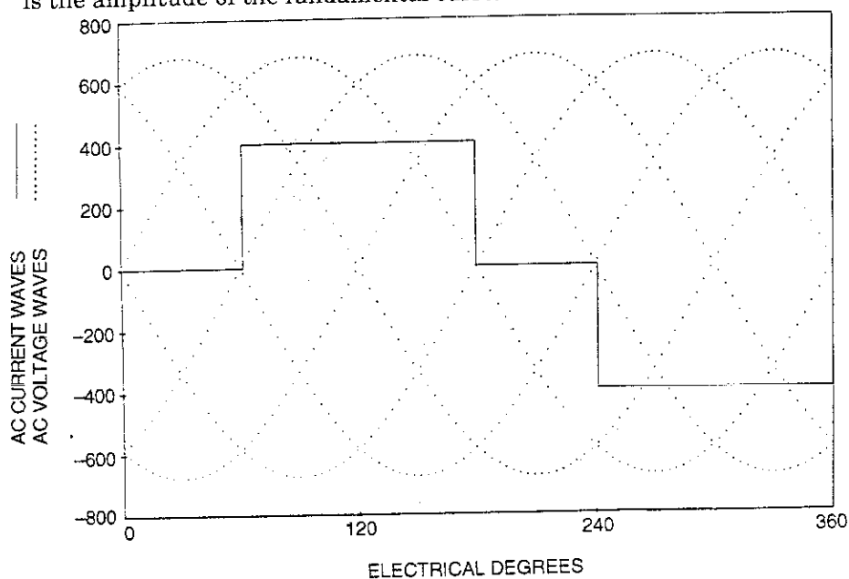
Fig 4.3 Ideal AC Current Waveform
