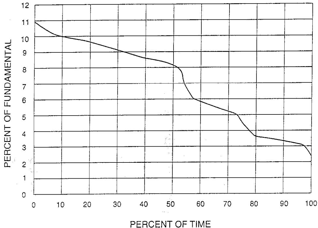
Fig 10.2 Probability Distribution of Current THD
