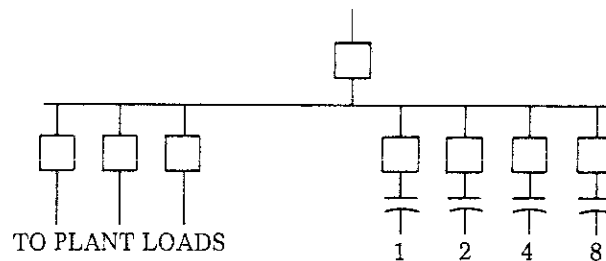
Fig 7.6 Capacitors Switched in Binary Values
