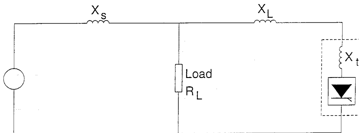
Fig 8.6 Impedance Diagram
