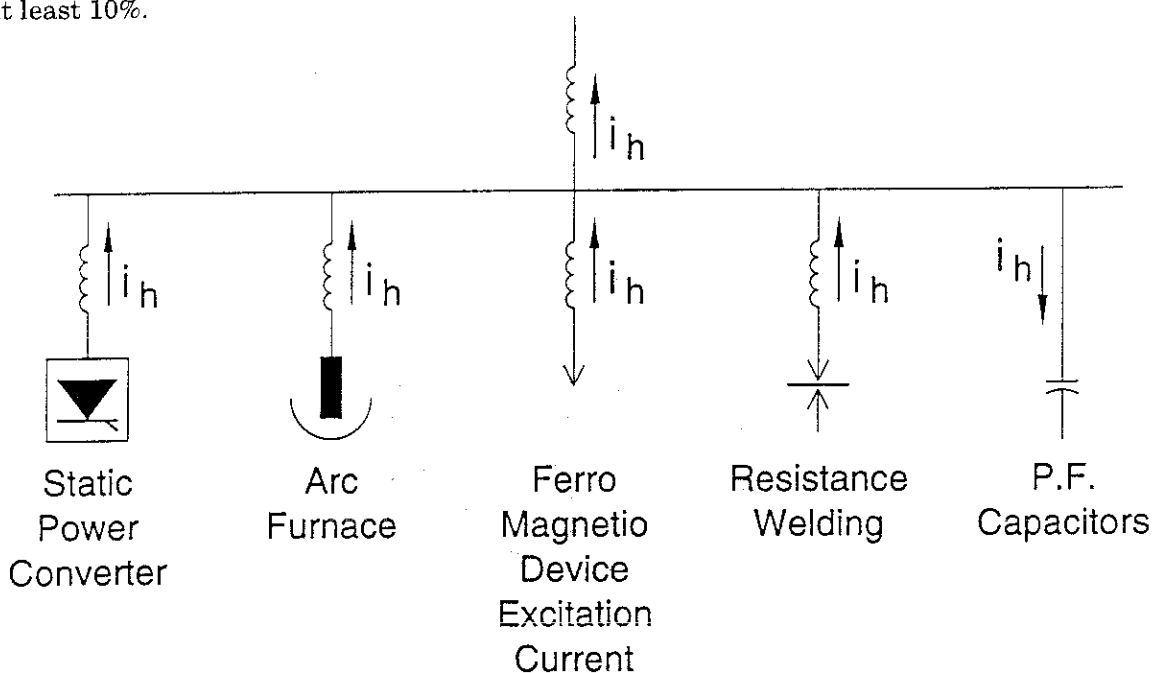
Fig 8.1 Modeling Nonlinear Loads by Current Sources
