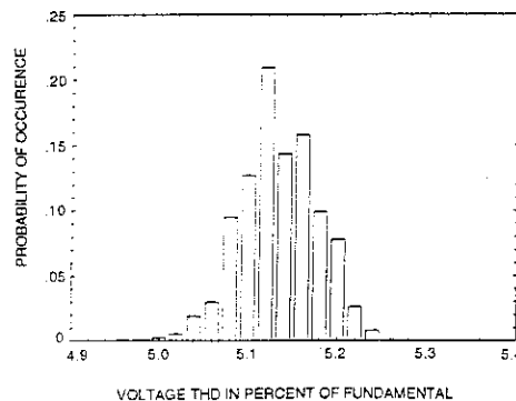
Fig 9.3 Harmonic Histogram of Voltage THD
