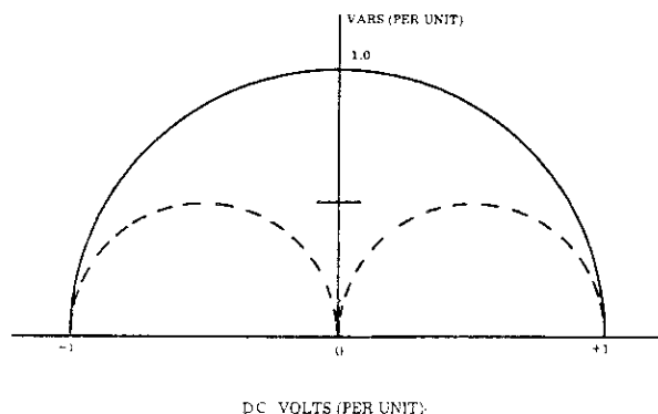
Fig 7.4 Reactive Power vs. DC Volts of Converter
