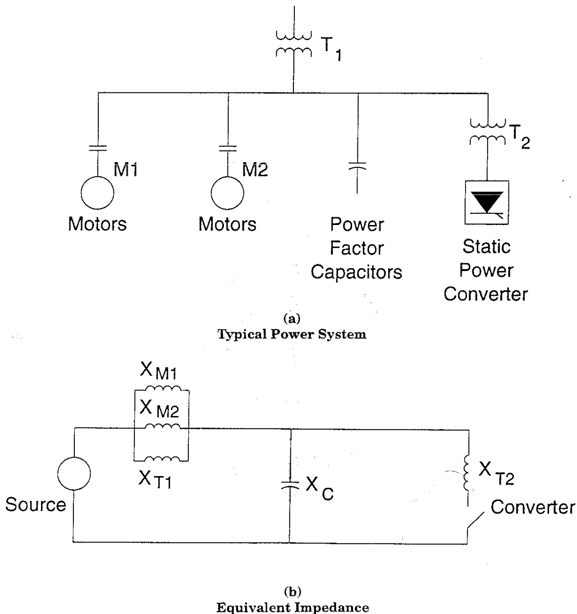
Fig 8.7 Typical Power System and Equivalent Impedance Diagrams
