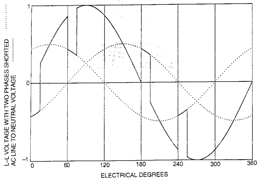
Fig 4.7 Rectifier Voltage Notching \alpha = 30^\circ
