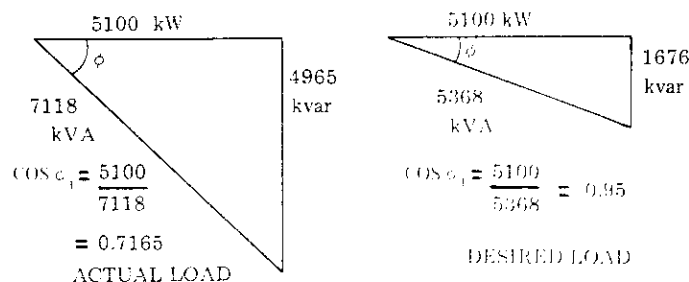
Fig 8.8 Power-Reactive Triangle for Power Factor Improvement
