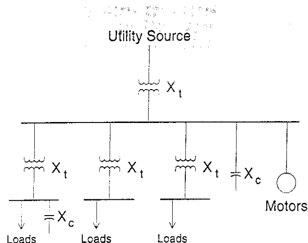
Fig 5.7 Typical Industrial Power System
