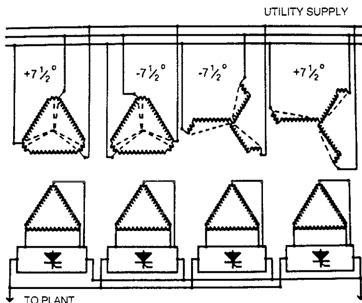
Fig 7.11 Transformer Connections for a 24-Pulse System
