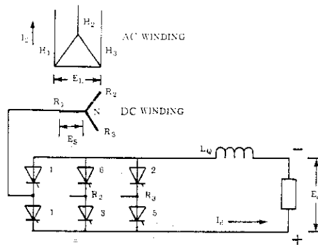
Fig 4.1 Three-Phase Bridge Rectifier Circuit
