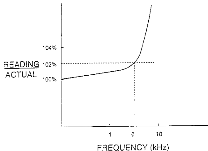
Fig 9.6 Potential Transformer Accuracy
