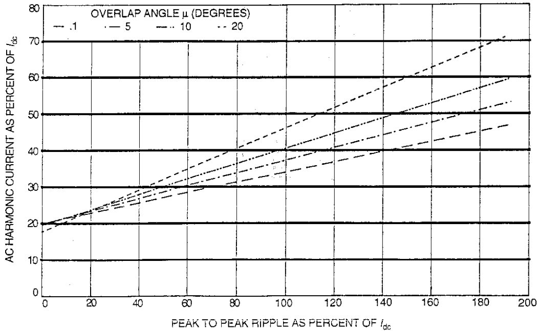
Fig 4.8 Six-Pulse Rectifier With DC Ripple Fifth Harmonic as a Function of DC Ripple
