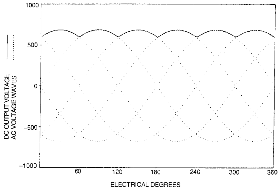
Fig 4.2 Ideal Rectifier Output Wave
