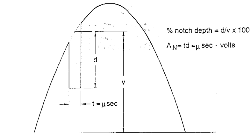
Fig 10.1 Definition of Notch Depth and Notch Area
