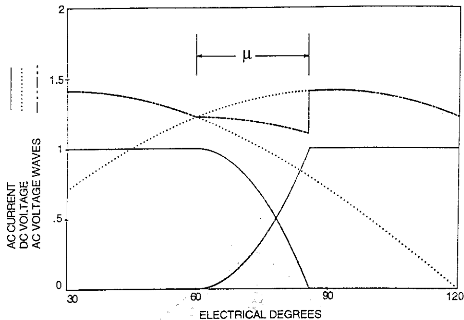
Fig 4.4 Commutation Overlap \alpha = 0^\circ , \mu = 25^\circ
